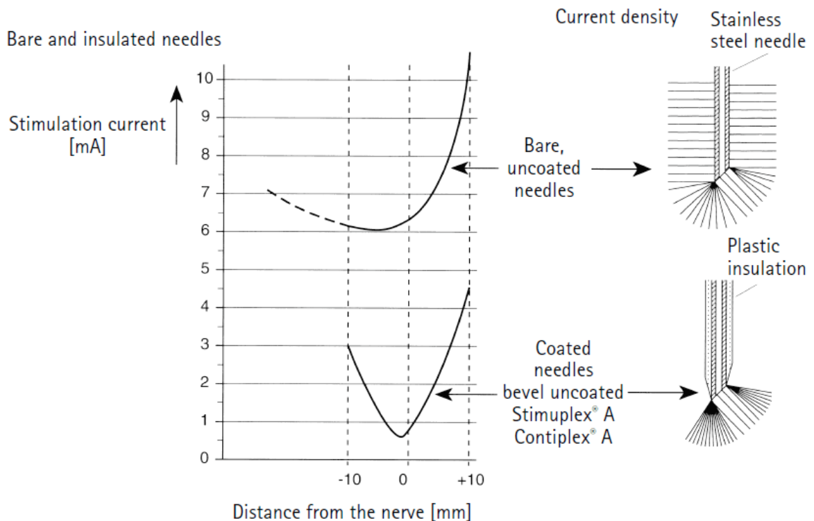
Figure 4. Comparison of non-insulated and insulated needle and their respective stimulation currents. (Reproduced from stimuplex HNS-11 manual with permission from B Braun, UK)
